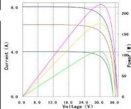
Current, power VS voltage characteristics (solar irradiant: 100%, 80%, 50%)
