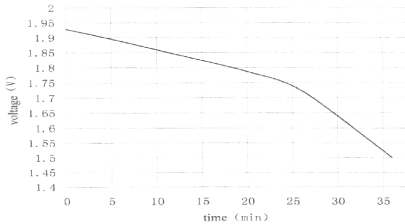
0.5hr disvcharge curve
