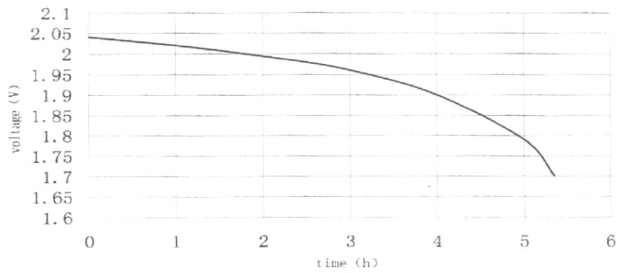
5hr discharge curve
