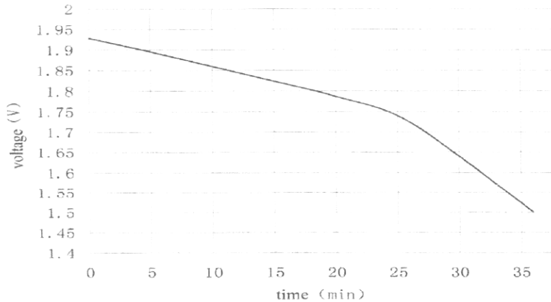
0.5hr discharge curve
