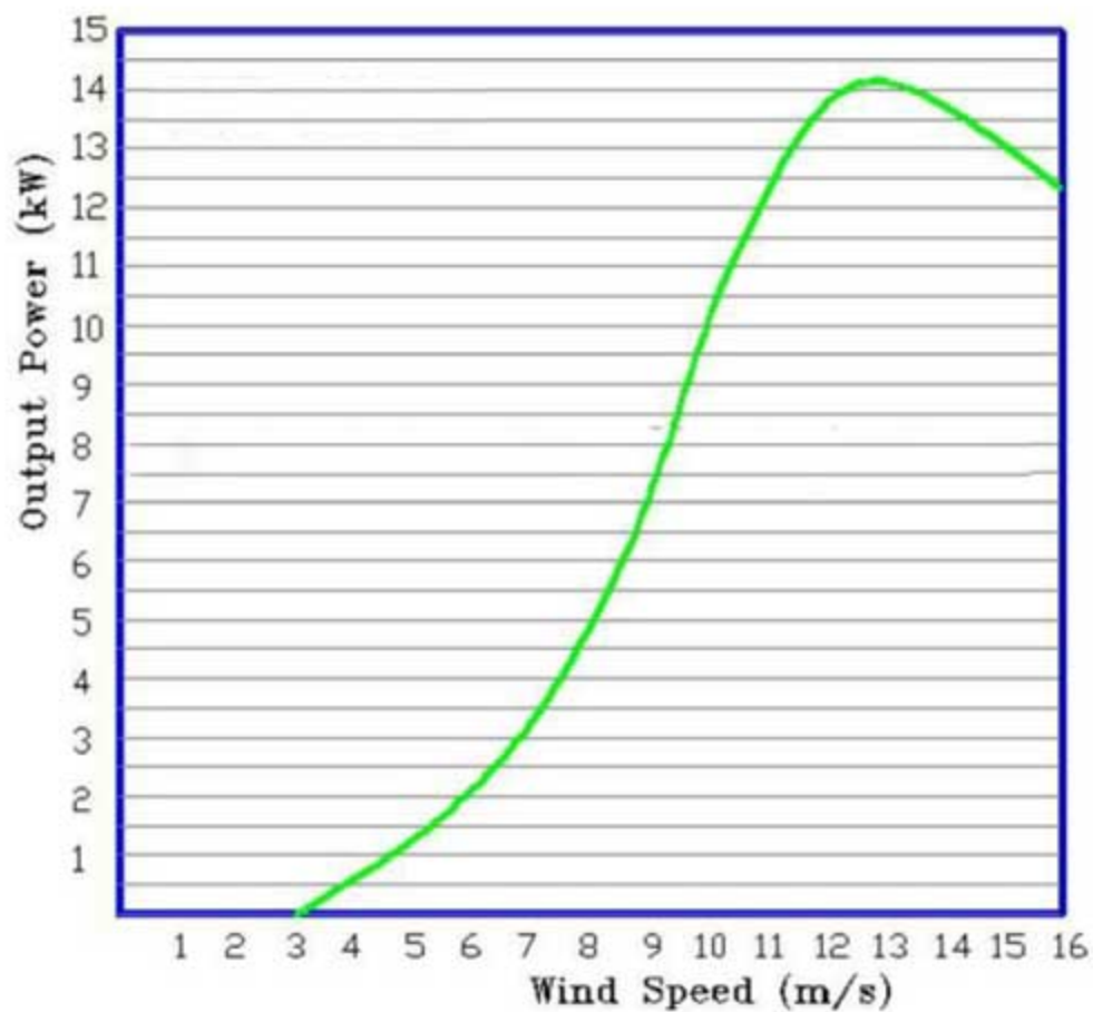
Output Power Curve - API-10KW-FREE
