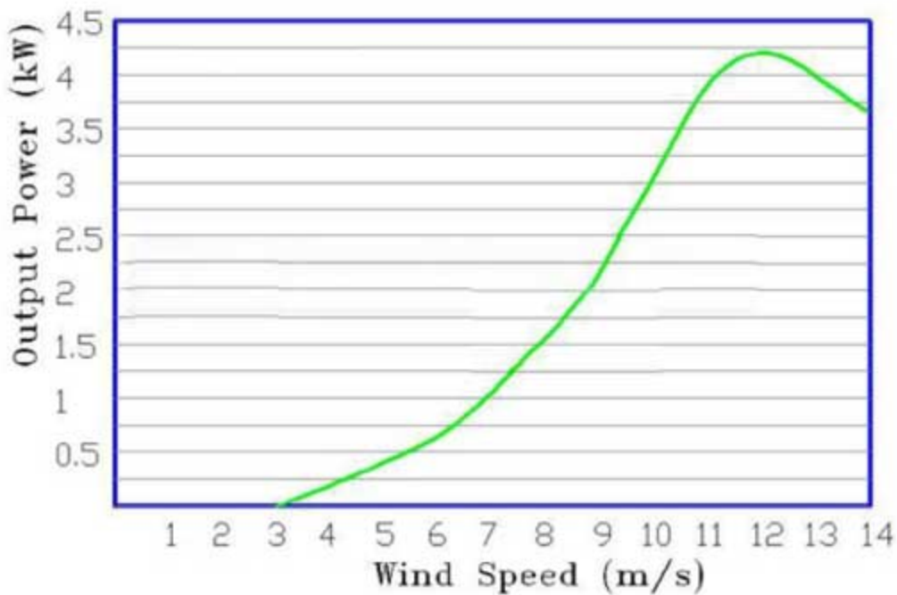
Output Power Curve – API-3KW-FREE
